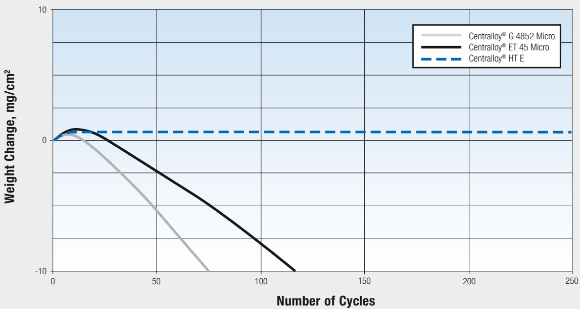
Cyclic Oxidation (45min at 1150°C, 15min at RT in air)
